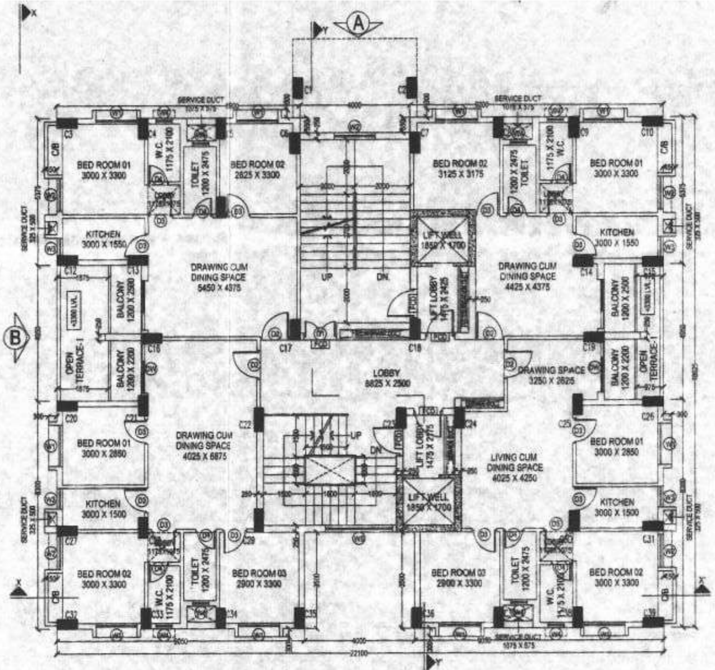
1ST. TO 3RD FLOOR PLAN SCALE- 1:100
